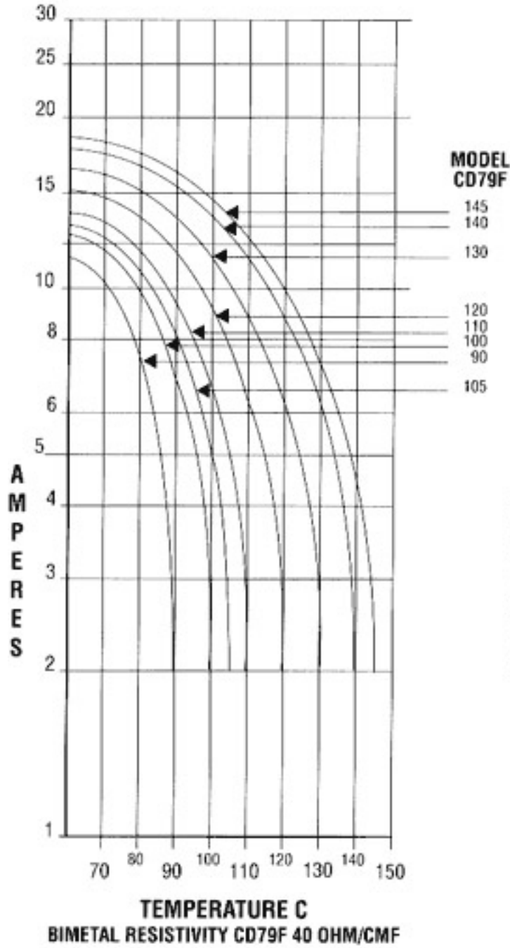
I- Tc Curve
