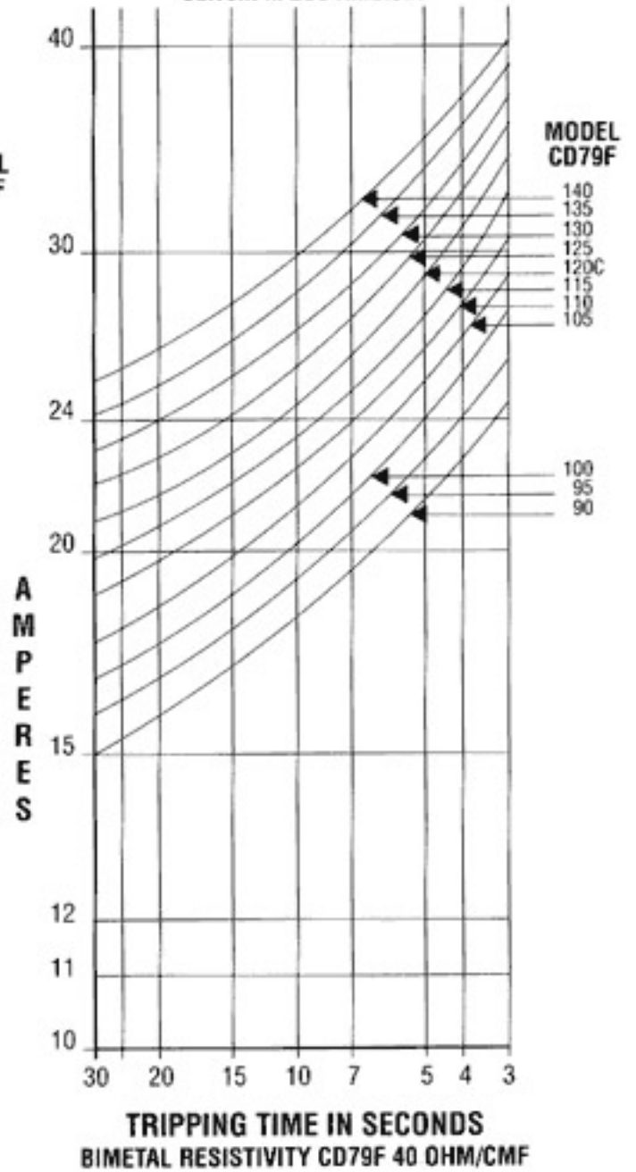
Average First Cycle Tripping Time (Second) VS Current in 25C Ambient
